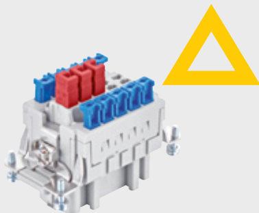
Delta connection
