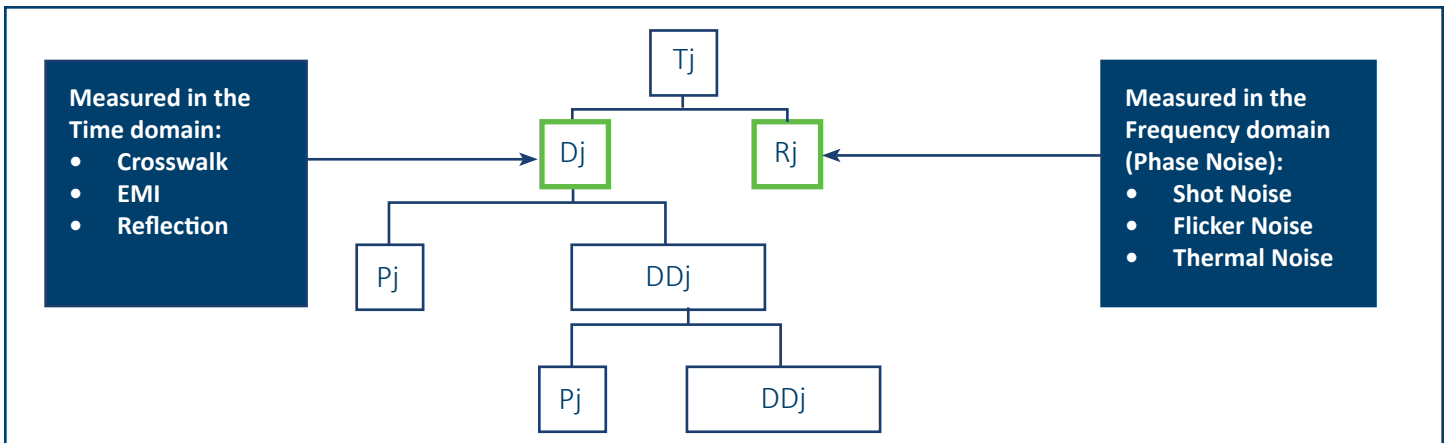
Figure 3: Total Jitter
